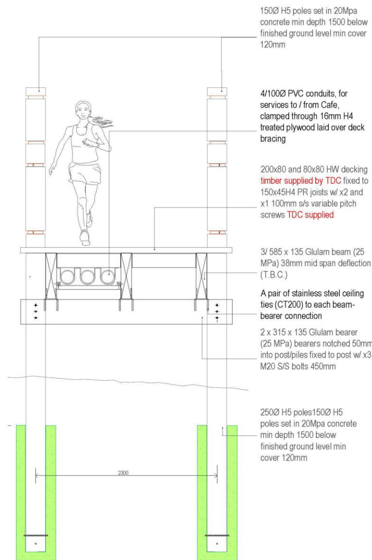
2 bridge (abudment) section 004
